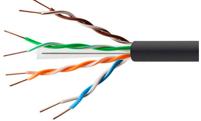
U/UTP CAT6 Outdoor Ethernet Cable
